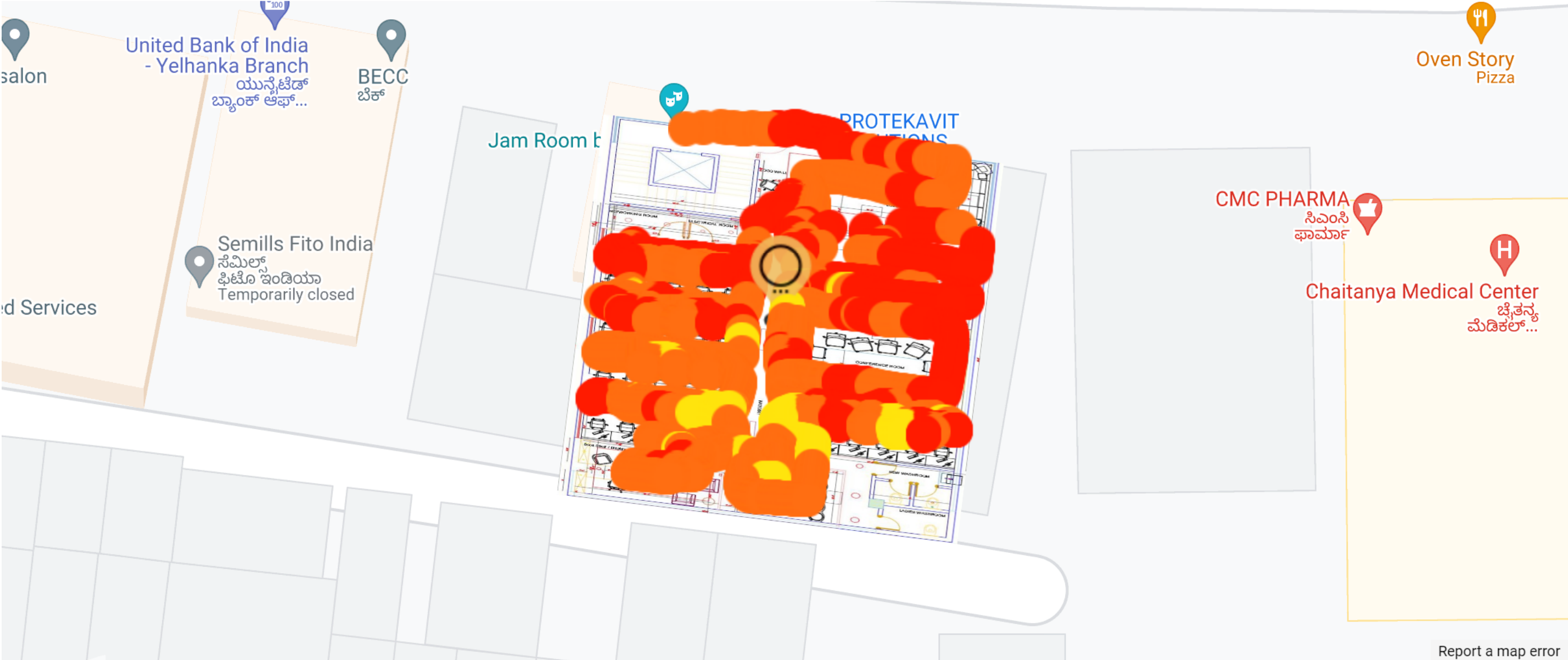
LTESNR KPI statistics per mobile operator for 405861_Jio True5G,40445_AIRTEL
