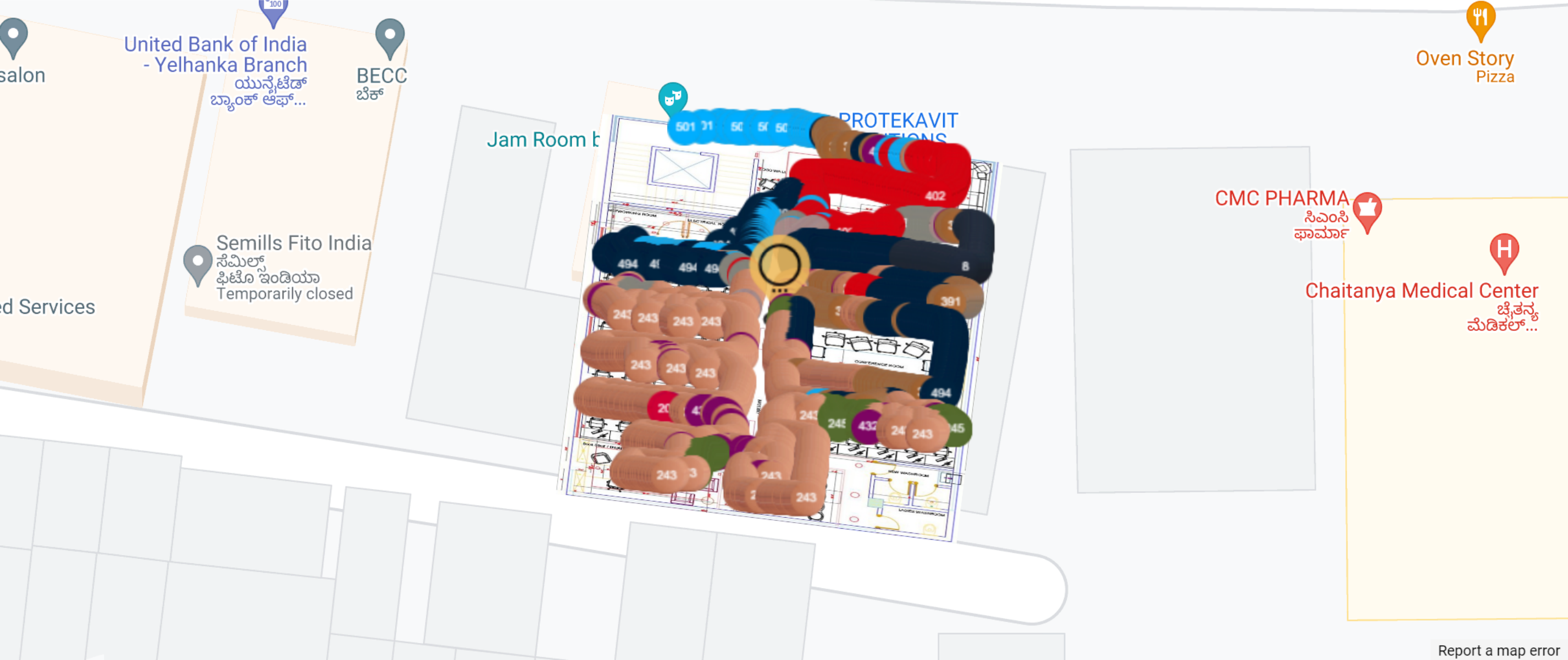
PCI KPI statistics per mobile operator for 405861_Jio True5G,40445_AIRTEL
